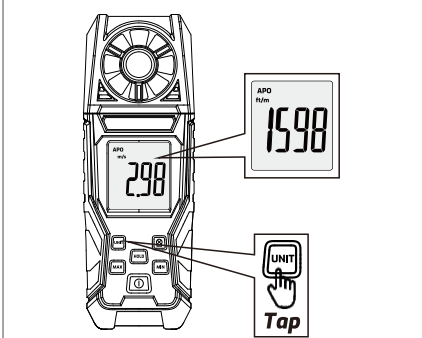
Air velocity unit (m/s, km/h, ft/m, mile/h, knots)
