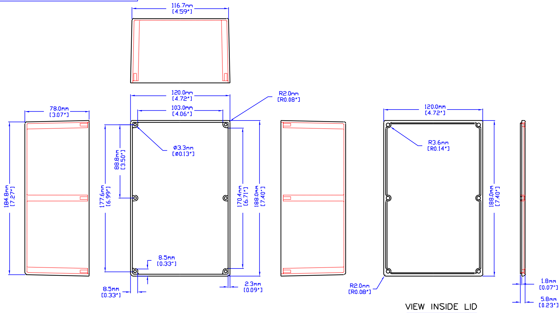
VIEW OF BOX (LID REMOVED)
