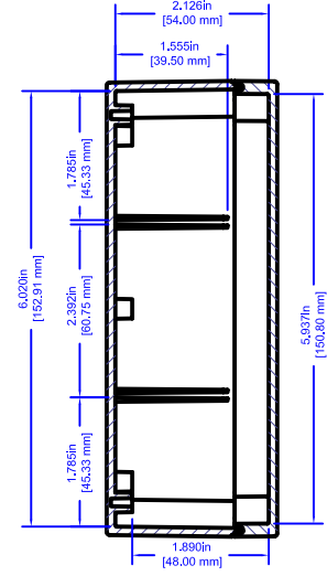
SECTION C-C SCALE 1 : 1
