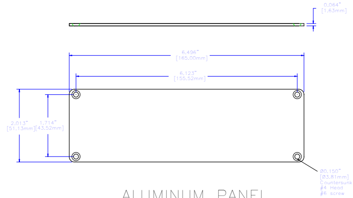
ALUMINUM PANEL
