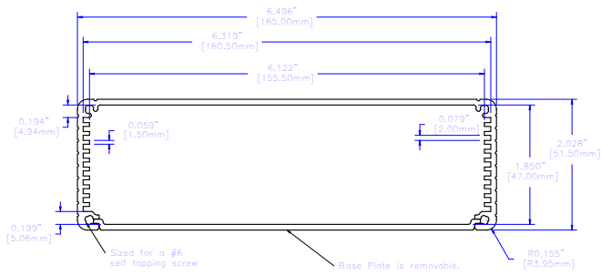
ALUMINUM EXTRUSION
