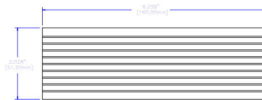
ALUMINUM EXTRUSION
