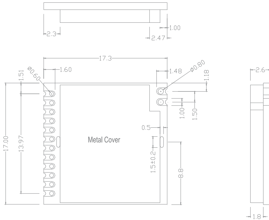
Figure 3: Mechanical Dimension
