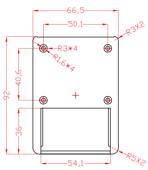
BASE
