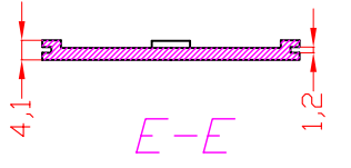
BATTERY-COVER
