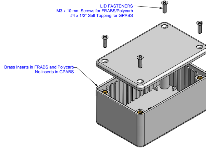
EXPLODED VIEW OF ASSEMBLY
