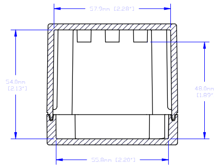
SECTION F-F SCALE 1 : 1
